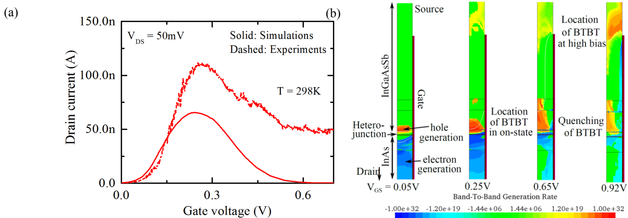
Figure 5. (a) Measured and simulated transfer characteristics over an extended gate voltage range. (b) Color-mapped diagram of the BTBT rate in the radial cross section of the nanowire TFET at different V_{GS} values ( V_{DS} = 50\text{mV} ). Quenching of BTBT generation at the hetero-junction causes negative transconductance.
