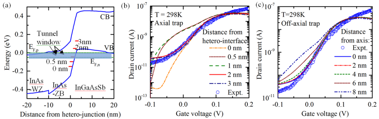
Figure 4. (a) Energetic and spatial location of the single trap leading to the I_D - V_{GS} characteristics by 3D simulations of the nanowire TFET shown in Fig. 1(a). (b) Variation of the location of single trap along the axis of the nanowire in segment R-1. (c) Variation of the location of the trap along the radius, at an axial distance of 2 nm.
