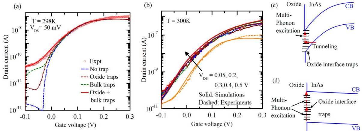
Figure 3. (a) Transfer characteristics of the TFET taking into account oxide and bulk traps separately. (b) Threshold voltage shift as observed in experiment with increasing V_{DS} is reproduced in the simulation. (c) Schematic diagram of trap-assisted tunneling and (d) multi-phonon excitation processes at the oxide/InAs interface.
