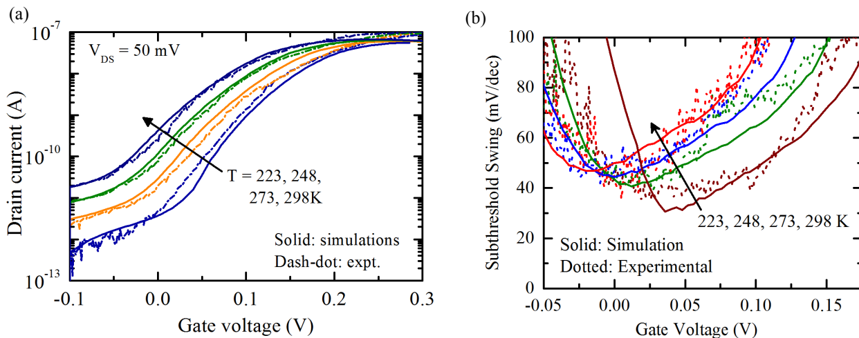
Figure 2. (a) Comparison of simulated temperature-dependent transfer characteristics of the TFET with the experimental data. (b) Comparison of SS calculated from the simulated and the experimental transfer characteristics. A reduction of the minimum swing with decreasing temperature is visible.
