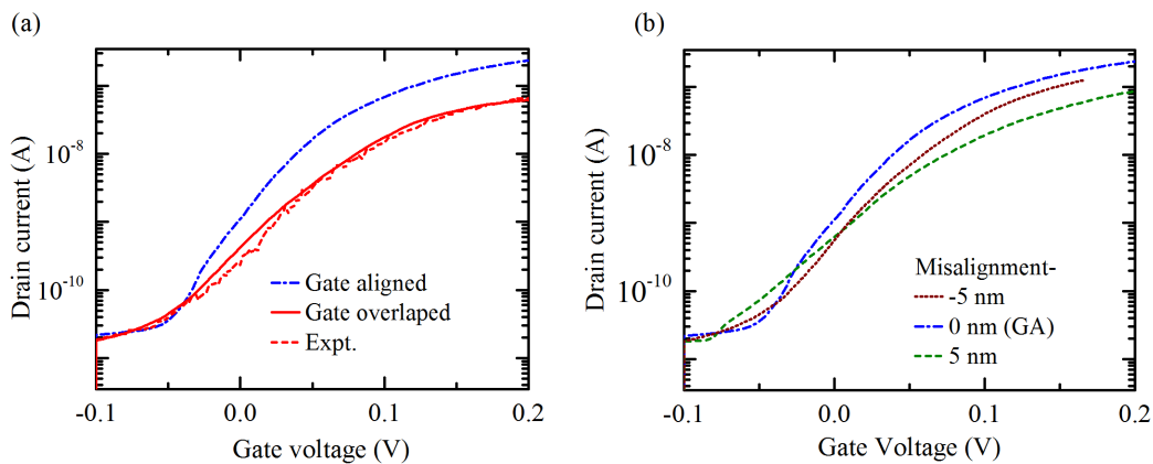
Figure 6. (a) Transfer characteristics of the nanowire TFET with the gate aligned to the InAs/InGaAsSb hetero-junction and with the gate overlapped on the source (present device geometry). (b) Impact of an overlap of 5 nm and an underlap of 5 nm on the transfer characteristics compared to the gate-aligned TFET.
