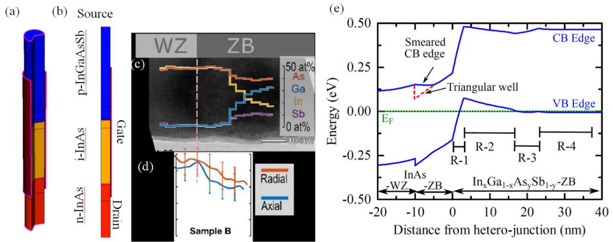
Figure 1. (a) Schematic of the simulated nanowire TFET, (b) radial cross section, (c) TEM image of the hetero-interface and material composition, (d) strain profiles, (e) band edge diagram along the axis of the nanowire at V_{DS} = V_{GS} = 0 V. A triangular-like quantum well is present at the InAs-ZB/InAs-WZ interface. Its effect on the band structure is mimicked by gradually changing the band gap of the material.
