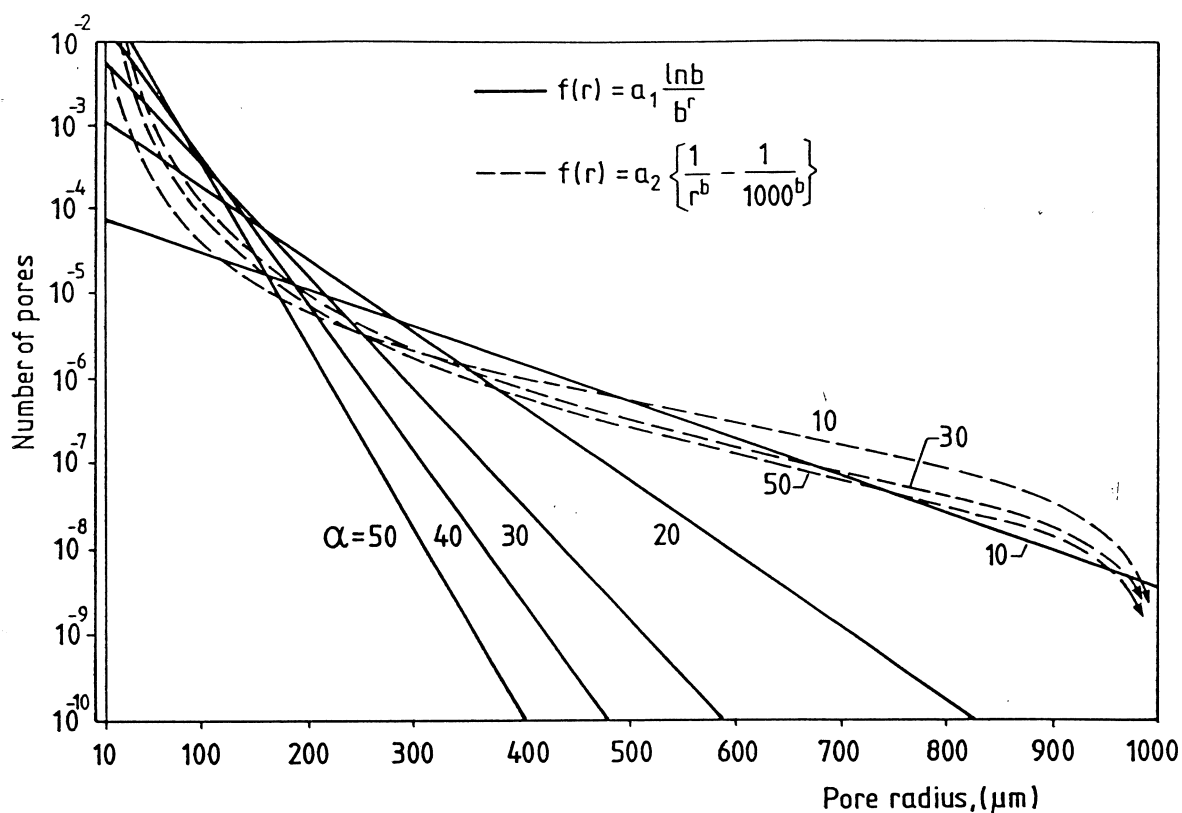
Fig 4.3: The frequency functions of the pore radius. Exponential function according to eq (4.20) and power function according to eq (4.35). The functions are normalized to equal total pore volume.
