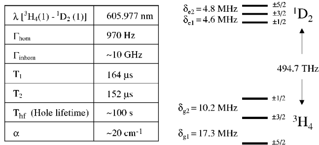
FIG. 4. Energy level diagram and relaxation data for the ^3H_4 - ^1D_2 transition of site I \text{Pr}^{3+} ions in Y_2SiO_5 . T_1 , T_2 , and \Gamma_{\text{hom}} are given according to Ref. 27.
