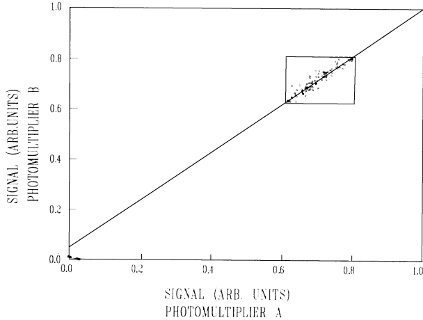
FIG. 4. Recording of dual detector data to which a linear fit has been performed as a “learning” curve.
