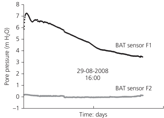
Figure 12. Pore pressure measurements on the Filborna landfill between 22 August and 3 September 2008
