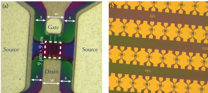
Figure 2.4: Micrographs of completed transistors using a 50\text{-}\Omega coplanar waveguide with a close-up showing a 9 \mu\text{m} \times 9 \mu\text{m} transistor cell in (a) and an overview with in total 27 transistors in (b).
