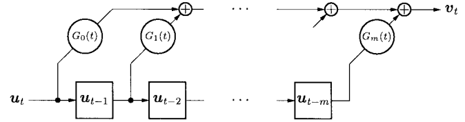
Fig. 4. A general time-varying polynomial convolutional encoder.
