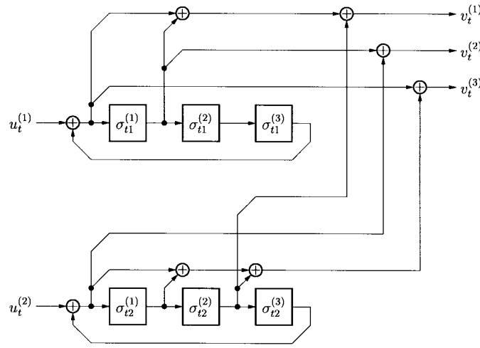
Fig. 1. The controller canonical form of the rate R = 2/3 generator matrix G(D) = \begin{pmatrix} \frac{1+D}{1+D^3} & \frac{D}{1+D^3} & \frac{1}{1+D^3} \\ \frac{D^2}{1+D^3} & \frac{1}{1+D^3} & \frac{1+D+D^2}{1+D^3} \end{pmatrix} .
