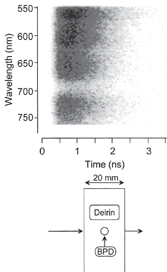
Fig. 4. 2D representation of experimental data on a Delrin sample of scattering plastic containing a cavity filled with the tumor sensitizing agent benzoporphyrine derivative (Quadralogics, Vancouver). The photon temporal dispersion as a function of the wavelength is shown with the absorption band of the benzoporphyrin molecules clearly visible.
