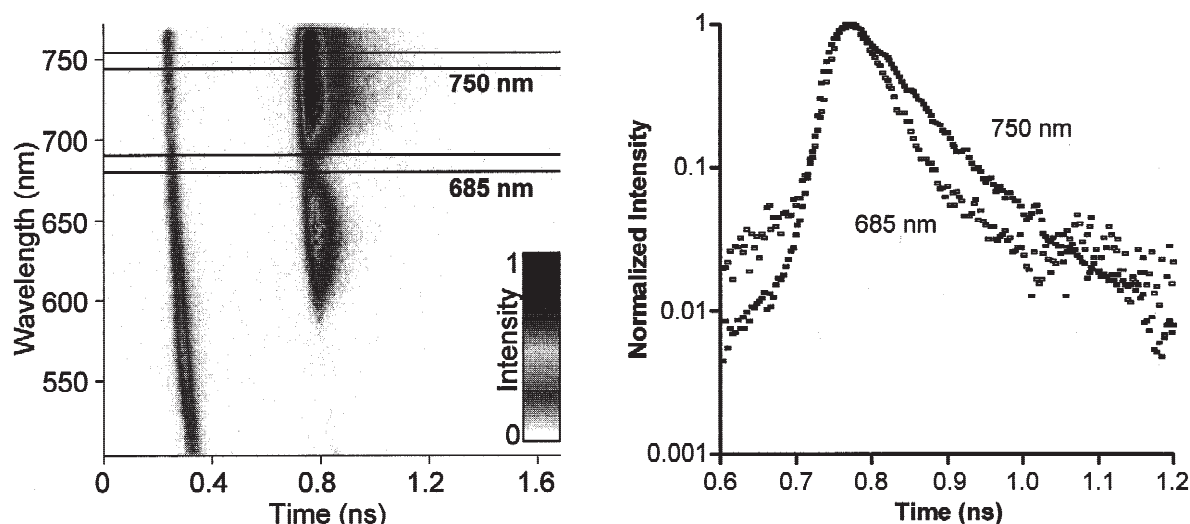
Fig. 5. 2D recording of white-light photons diffusely scattered through rat tissue loaded with disulphonated aluminium phthalocyanine. Transmission and receiving fibers were separated by 8 mm. Dispersion curves taken for two narrow wavelength regions, on and off the sensitizer absorption are shown, featuring different behaviors (from af Klinteberg et al. , 1999).
