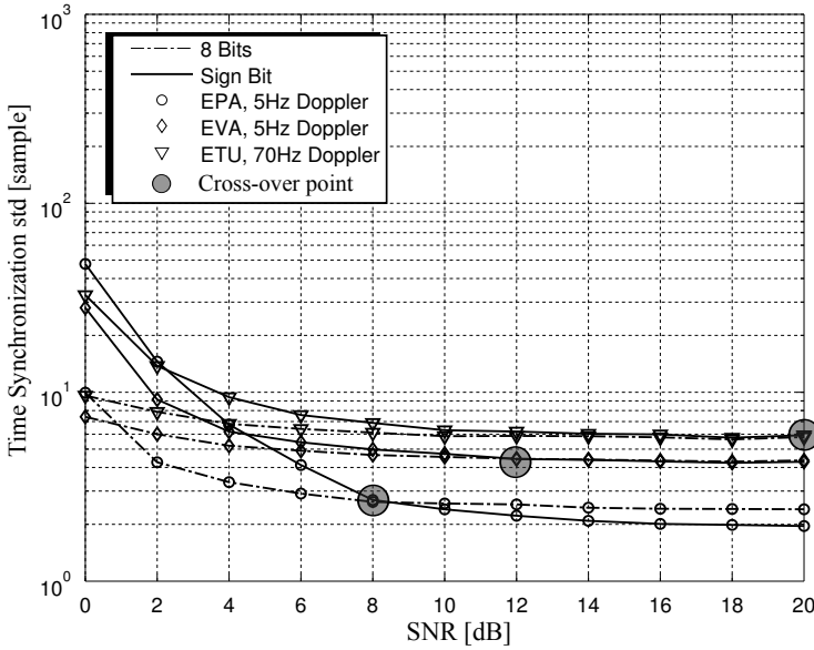
Figure 5.4.: Symbol timing standard deviation for EPA, EVA and ETU channel models as a function of SNR.
