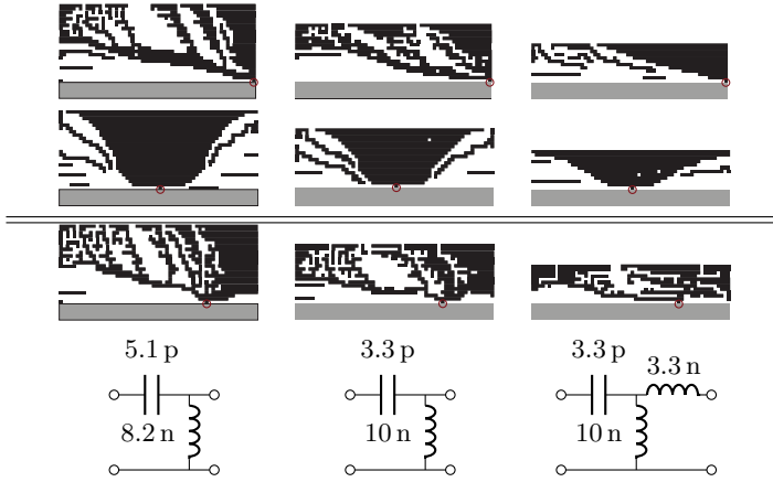
Figure 15: Antenna regions, black, of structures optimized for simultaneous multiband minimum Q . Circled—fed mesh edges on the borderline between antenna region and ground plane, at the side of the model in the w -direction (first row from the top), in the center (second row), and half way between center and side (third row). Bottom row—matching networks for the structures on the third row from the top, in SI units. Gray shaded—part of the ground plane. From left to right columns correspond to antenna regions extending 20 %, 15 %, and 10 % of the entire device model, at one end in the \ell -direction, as depicted in Fig. 8b.
