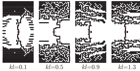
Figure 5: Four of the structures simulated in Efield whose Q -factors are depicted in Fig. 3. Feeding edges are circled.
