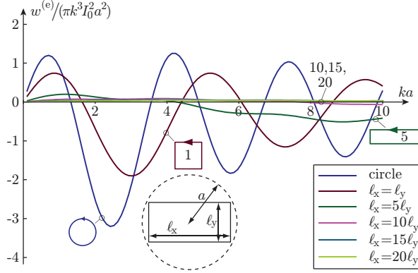
Figure 11: Stored electric energy for circular (A.1) and rectangular loop currents.
