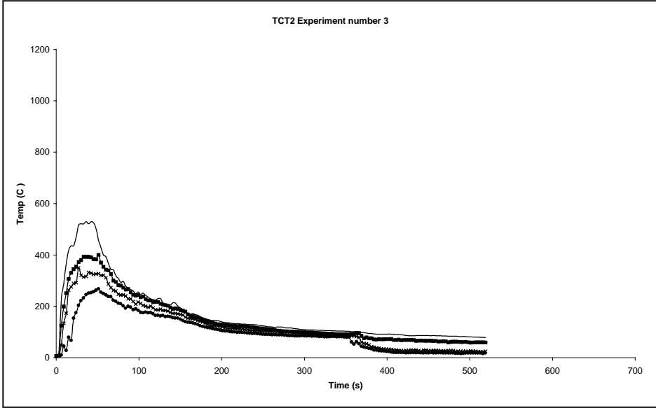
Figure A6. Temperature-time graph for experiment number 3.
