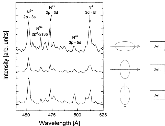
FIG. 13. Comparison of nitrogen spectra in the region of transitions between excited lithiumlike states. The three spectra are obtained using a gas jet with an oval cross section of 400 and 800 \mu\text{m} extension, respectively. A transverse spectrum and two longitudinal spectra (along the short and long dimensions of the gas jet) are displayed, as indicated by the symbols alongside each spectrum. Gain lines are indicated by arrows.
