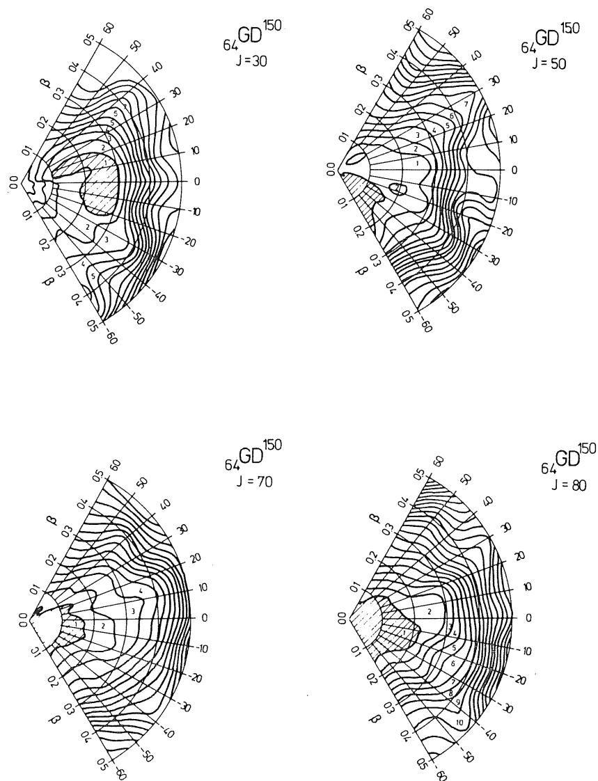
Fig. 3. The deformation energy surfaces obtained for ^{150}\text{Gd} for angular momenta I = 30\hbar , 50\hbar , 70\hbar and 80\hbar . For details see caption of fig. 2.
