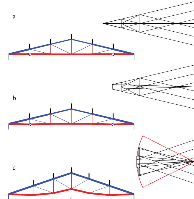
Fig. 10. (a) Gable truss with varying force magnitude in chords. (b) Vertices marked with F in the force diagram are translated slightly downwards, the forces in the connecting vertical edges are no longer zero. (c) Design of a constant-force gable truss.
