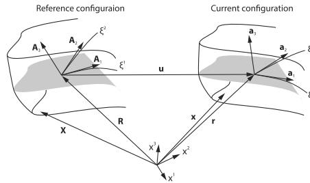
Fig. 2. Membrane kinematics.
