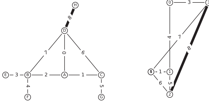
Figure 7.10: The structure in the form diagram to the left has an edge (edge zero) with zero force magnitude.
