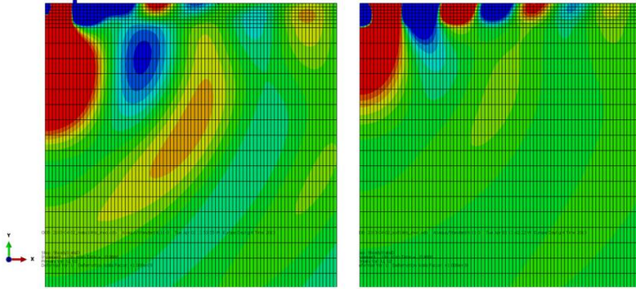
Figure 3: Vertical displacement amplitude of (left) soil model with mass \rho = 8271 \text{ kg/m}^3 and (right) model with no mass, for a prescribed harmonic load with excitation frequency 14Hz and unit amplitude. Surface waves are reduced (left) due to the mass on top of the surface.
