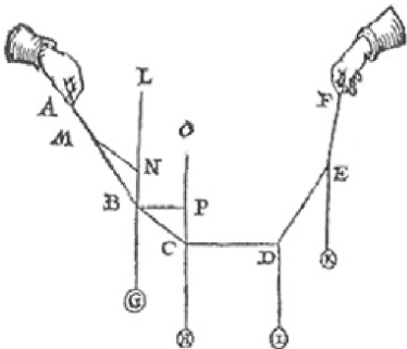
Figure 7.2: Stevin’s drawing of force equilibrium [96].
