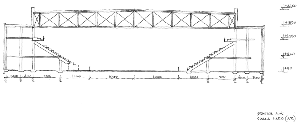
SEKCTION A-A – Section drawing A-A
