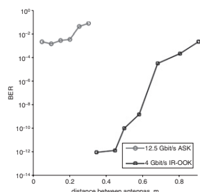
Fig. 3 BER for 4 Gbit/s using impulse radio OOK and 12.5 Gbit/s using binary ASK for different distances between Tx and Rx antennas
