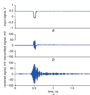
Fig. 2 Input signal of wavelet generator (Fig. 2a); on-chip measurement of generated signal (Fig. 2b) (centre frequency of wavelet is 59 GHz, de-embedded voltage swing is 177 mV pp ; pulse length of baseband signal is 53.9 ps, wavelet is 56.4 ps); received wavelet after transmission (Fig. 1c)
