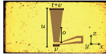
Fig. 4. Optical micrograph of a slot feed with coplanar waveguide input in a groundplane on a 1300 \times 650 \mu\text{m}^2 GaAs DRA, also shown are definitions for slot dimensions.
