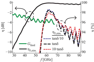
Fig. 8. Simulated radiation efficiency \eta_{5,\text{sim}} of the DRA for a \tan \delta of different orders of magnitude. Notice that the simulated efficiency for the estimated value of tangential loss is plotted twice, scaled in both dB and %. Also shown is the insertion gain of the assembly feed line G_{\text{feed}} , estimated from measurements.
