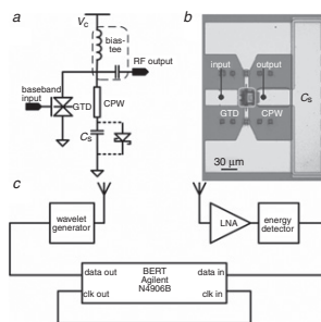
Fig. 1 Transmitter circuit schematics of wavelet generator, chip photo, and system description
