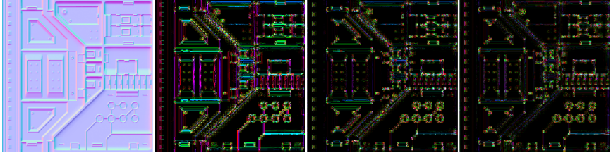
Figure 5: False color images of the pixel errors: From left to right: Original map, 3Dc, e3Dc and TF. We can clearly see improved performance of the TF algorithm over the two 3Dc compressor variants.
