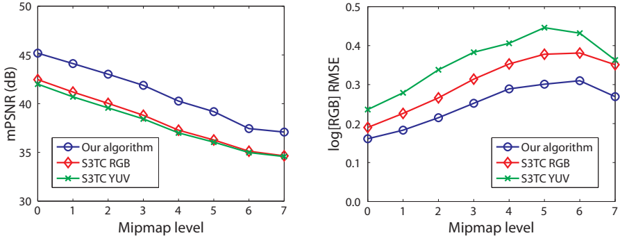
Figure 15: Here, the average mPSNR and \log[\text{RGB}] RMSE values are presented for various mipmap levels of our test images, where 0 is the original image and higher numbers are sub-sampled versions.
