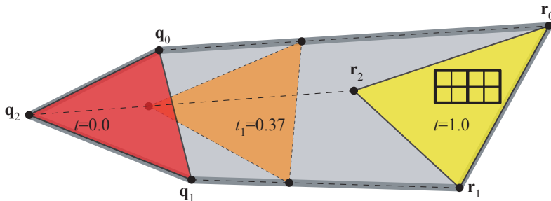
Figure 1: A time-continuous triangle (TCT) defined by a starting triangle, \Delta\mathbf{q}_0\mathbf{q}_1\mathbf{q}_2 , at t = 0 , and an ending triangle, \Delta\mathbf{r}_0\mathbf{r}_1\mathbf{r}_2 , at t = 1 . The TCT is simply the continuous set of linearly interpolated triangles between t = 0 and t = 1 .
