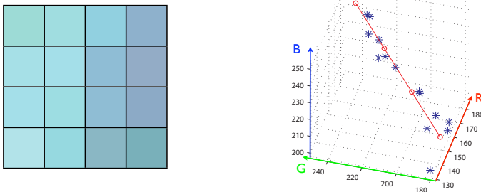
Figure 9: S3 texture compression (S3TC/DXTC) illustrated. The color values in RGB triples from a block of 4 \times 4 texels are plotted in a Cartesian coordinate system, and a line is fitted to the points. In the compression stage, each texel (blue stars) is assigned to one of four quantized positions (red circles) along this line.
