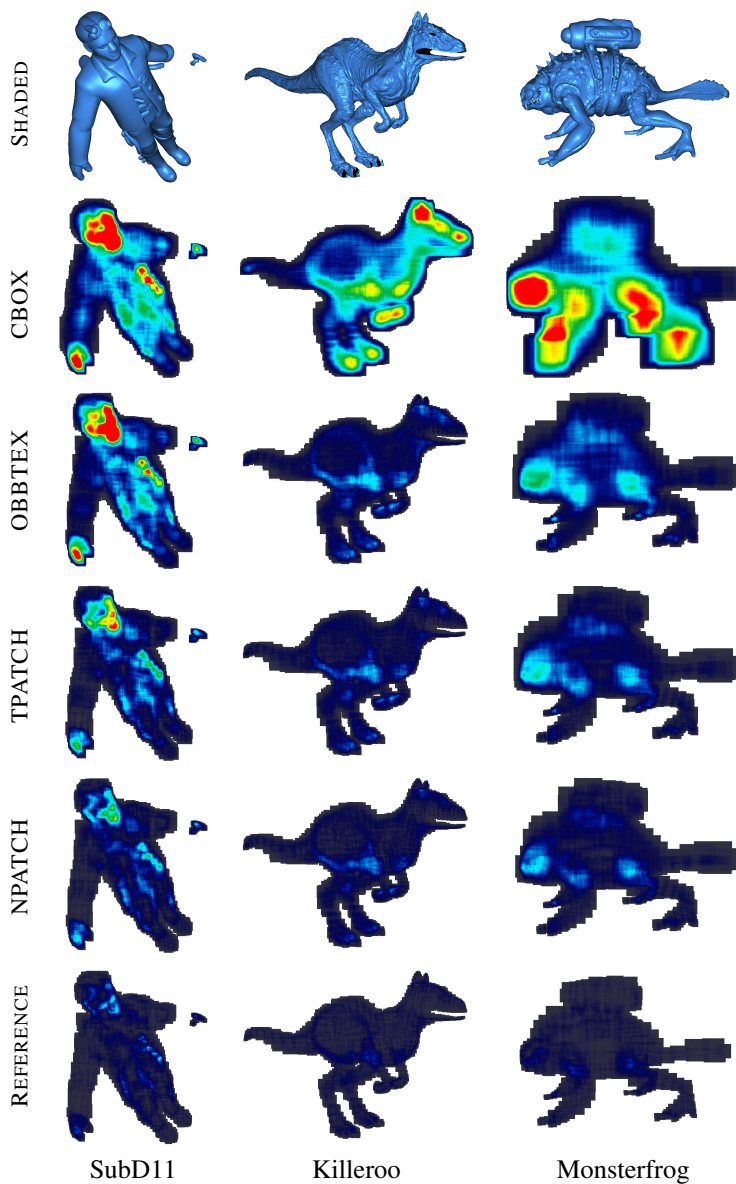
Figure 11: False color images that show the bounding box overlap in screen space. Red means 128 or more overlapping bounding boxes. For the SubD11 mesh, a constant displacement is added to the base mesh in the base patch’s normal direction. For the Killeroo and Monsterfrog meshes, the original displacement maps are used.
