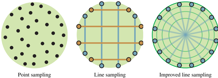
Figure 9: DOF sampling patterns
