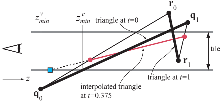
Figure 5: A time continuous triangle (TCT) defined by a starting triangle, \Delta \mathbf{q}_0 \mathbf{q}_1 \mathbf{q}_2 , and an ending triangle, \Delta \mathbf{r}_0 \mathbf{r}_1 \mathbf{r}_2 , here shown in two dimensions. Due to that these triangles do not have the same orientation, problems in Zmax-culling can occur. Normally, we compute z_{min}^{tri} = \max(z_{min}^v, z_{min}^c) . In this case, this is not correct, since at, e.g., t = 0.375 , the true depth at the tile corner (blue square) is smaller than z_{min}^c which is computed using the plane equations of the two triangles of the TCT. Our solution is simply to use z_{min}^{tri} = z_{min}^v when the orientation of the triangles changes. This gives a conservative estimate.
