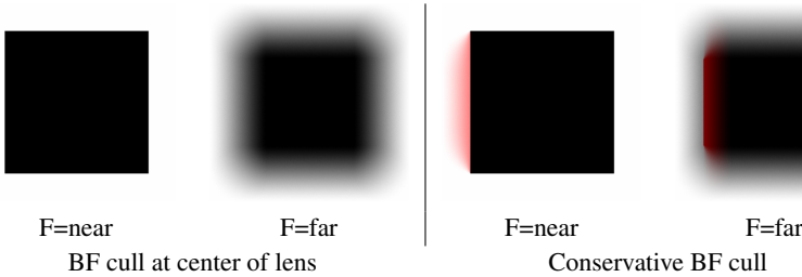
Figure 3: A red cube with a black front face is rendered with depth of field. Focus is set at the front and back of the cube. The cube is positioned so that the left face has a normal perpendicular to the view vector at the center of the lens. The left face can thus be backface culled for that camera position. For rays starting slightly off-center, the left (red) side is visible, and contributes to the final image. The two leftmost images show the result when the backface test is done only at the center of the lens, and the two rightmost images the reference result.
