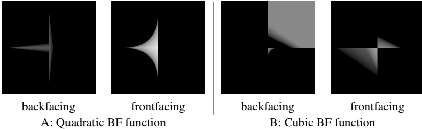
Figure 2: Motion blur rasterized triangles. The shutter is open in t \in [0, 1] . A: The triangle moving according to Equation 1 is rasterized on screen with \alpha = 0.1 and \beta = 0.9 , where the triangle is backfacing at t = 0 and t = 1 . The left image shows the covered samples for the backfacing region, while the right image shows the covered samples for the frontfacing region. Note that with naïve backface culling, all the covered samples to the right will be missed, which is incorrect. B: The triangle moving according to Equation 3 flips from front to backfacing (or vice versa) three times in the time interval. The left image shows a rendering of the backfacing region, and the right image shows the frontfacing region.
