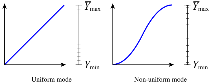
Figure 3: The two luminance quantization modes. The non-uniform mode is used for better handling tiles with sharp luminance transitions, such as edges.
