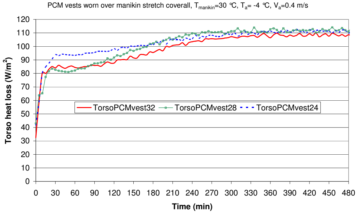
Fig. 2. Heating effects of the PCM vests ( T_{\text{melt}}=32, 28 and 24\text{ }^{\circ}\text{C} ) on the manikin in the subzero environment.
