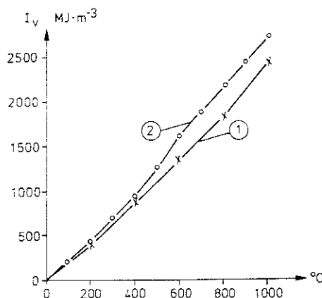
Figure 4.2.2a. Volumetric enthalpy I_v as a function of temperature for concrete with granite aggregate. (1) Measured curve under cooling (corresponding to the c_p values in table 4.2.2a), (2) theoretical curve
