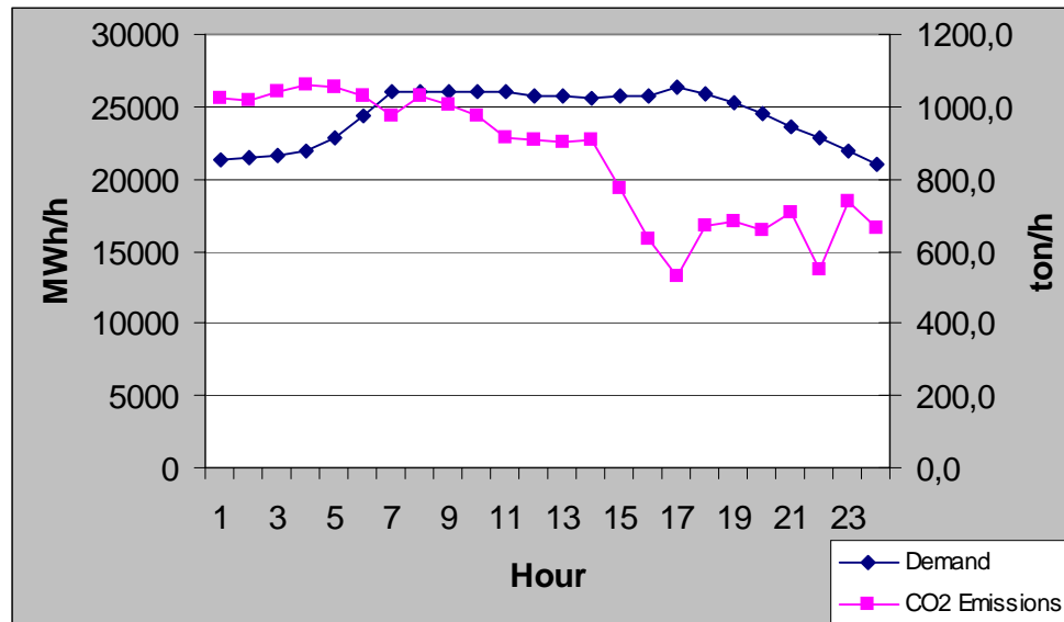
Figure 2.14. Demand and CO 2 emissions Feb. 5, 2001
