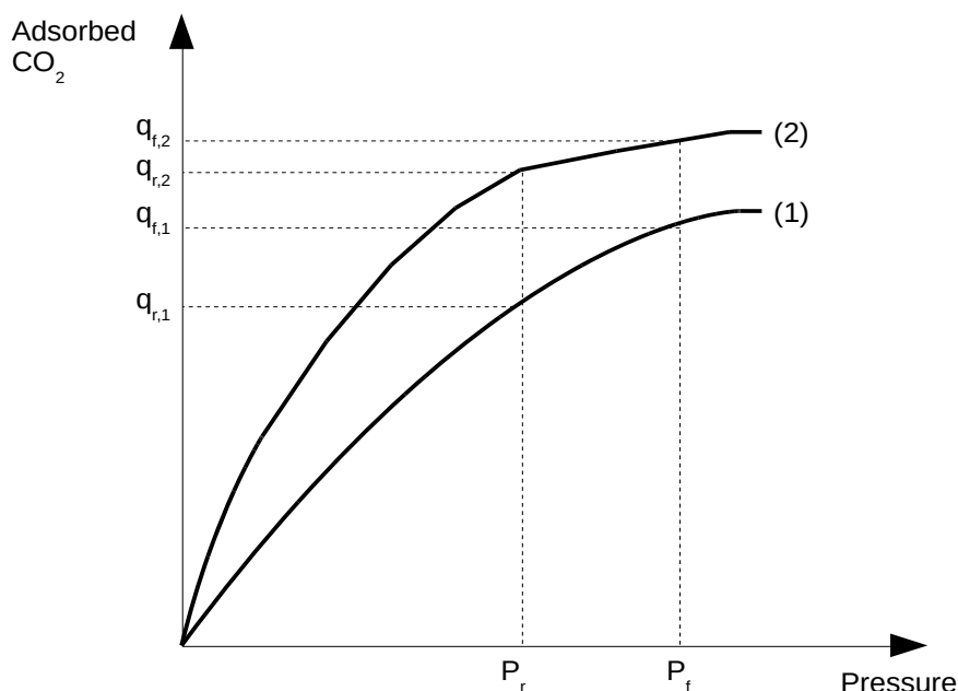
Figure 9 Two generic adsorbant isotherms showing the partial pressure of CO 2 in the gas streams at feed pressure (high) and regeneration pressure (low). \Delta q equals the separating capacity for one column cycle. Image adapted from (Grande 2011).
