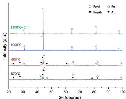
Fig. 12. Diffraction pattern of compacted samples (with fine iron and aluminum particles) after heating at 7.5\text{ }^{\circ}\text{C min}^{-1} to different temperatures.
