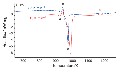
Fig. 6 DSC plots for Ti + Al samples
