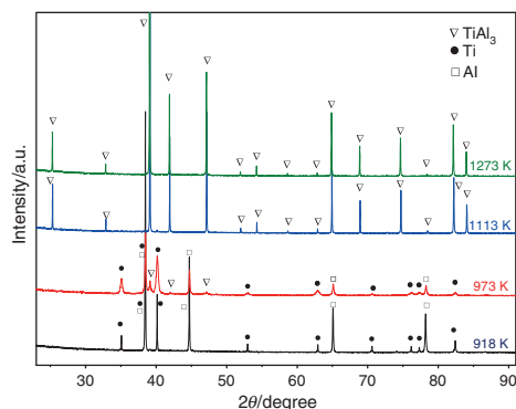
Fig. 3 Diffractograms of Ti + 3Al samples heated to different temperatures (15 K min -1 )
