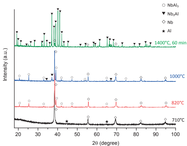
Fig. 13. Diffractograms of Nb-33.3at.%Al samples heated to different temperatures at 15^\circ\text{C min}^{-1} .
