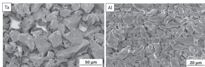
Fig. 2. SEM images of tantalum (<75 µm) and aluminum (<60 µm) powders.
