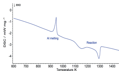
Fig. 3. DSC plot for Ta+3Al sample heated at 15 \text{ K min}^{-1} .
