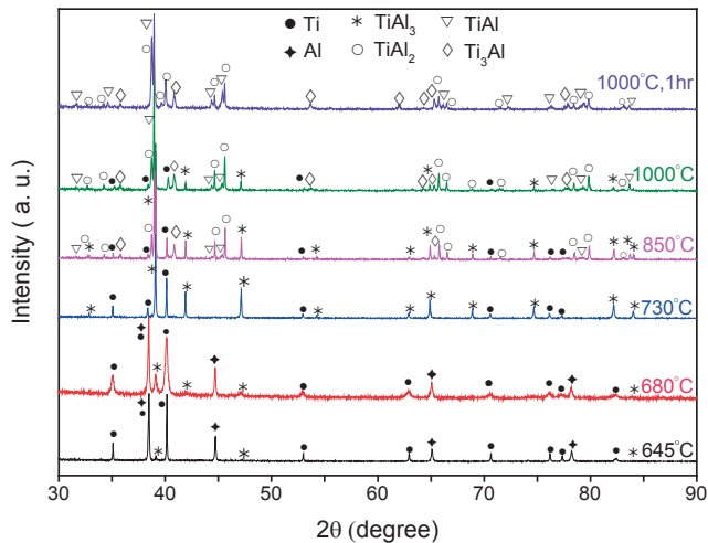
Fig. 8. Diffractograms of Ti-50at.%Al samples heated to different temperature at 15^\circ\text{C min}^{-1} .
