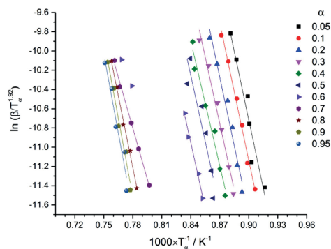
Fig. 13. Starlink isoconversion plots for the determination of apparent activation energies at different degrees of conversion to \text{Al}_3\text{Ta} .
