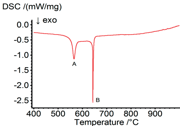
Fig. 9. DSC plot of the Fe-40at.%Al sample heated to 1000°C at 7.5°C min -1 .
