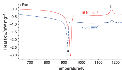
Fig. 9 DSC plots for 3Ti + Al samples
