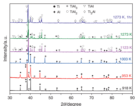
Fig. 7 Diffraction patterns of Ti + Al samples heated to different temperatures (15 K min -1 )
