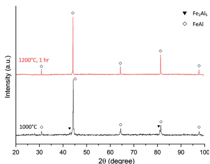
Fig. 8. Diffractogram of compacted samples (with coarse iron and fine aluminum particles) heated at 7.5\text{ }^{\circ}\text{C min}^{-1} to 1000\text{ }^{\circ}\text{C} and above.
