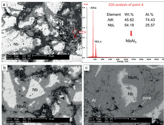
Fig. 5. SEM micrographs of Nb + 3Al samples (with fine Al particles) heated at 15 °C min -1 to (a) 815 °C + cooled, (b) 850 °C + cooled, (c) 850 °C + 15 min + cooled (30 °C min -1 ).
