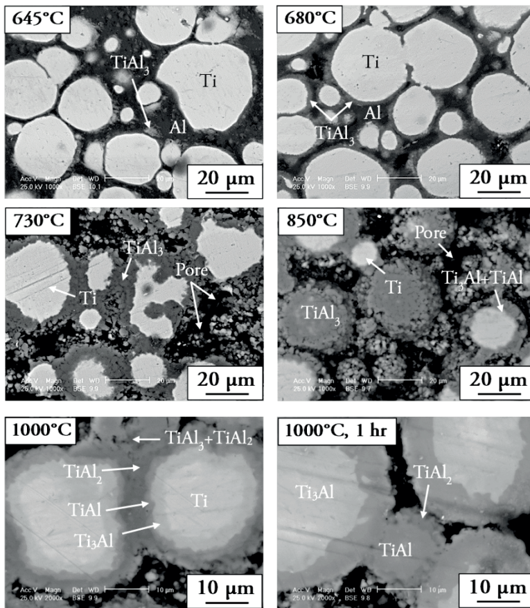
Fig. 7. SEM images of Ti-50at.%Al samples heated to selected temperatures at 15^\circ\text{C min}^{-1} .
