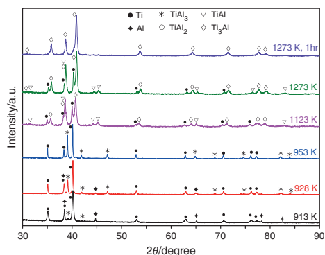
Fig. 10 Diffraction patterns of 3Ti + Al samples heated to different temperatures ( 15 \text{ K min}^{-1} )
