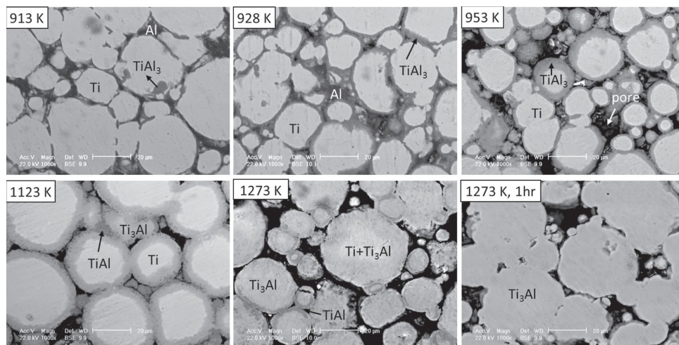
Fig. 11 SEM micrographs of 3\text{Ti} + \text{Al} samples heated to different temperatures ( 15 \text{ K min}^{-1} )
