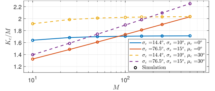
Fig. 4. Normalized MRC interference power.
