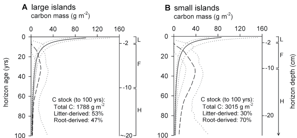
Figure 13: Northern Sweden island chronosequence ( Paper IV ). Carbon (C) dynamics in vertically stratified organic horizons of forested islands. Model estimates of C from aboveground litter (solid lines) and C introduced belowground via root transport (broken lines). Carbon mass was modeled to a horizon age of 100 years based on C mass and ^{14}\text{C} measurements in profiles from three large (A, representing early succession) and three small (B representing late succession) islands. Solid lines show means and dotted lines show the 95 % central credibility intervals. The posterior probability that the root-derived fraction is larger in small islands than in large islands is 0.97. Approximate depths are indicated for transitions between the main categories of horizons sampled; L: litter; F: fragmented litter; H: humus.
