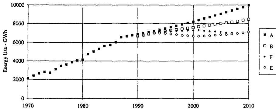
Figure 2. Ventilation, Cooling and Kitchen End-Uses. The scenarios are: A) all new and replacement equipment continues to have the same energy-efficiency as 1990 models; B) reference case, with efficiency improvements implemented according to present trends and investment payback criteria, 25 percent electric price increase; E) full implementation of utility-sponsored DSM incentives, with all programs beginning in 1994; F) full implementation of DSM incentives, with programs for new and replacement equipment beginning in 1994 and retrofit programs delayed until 2000.
