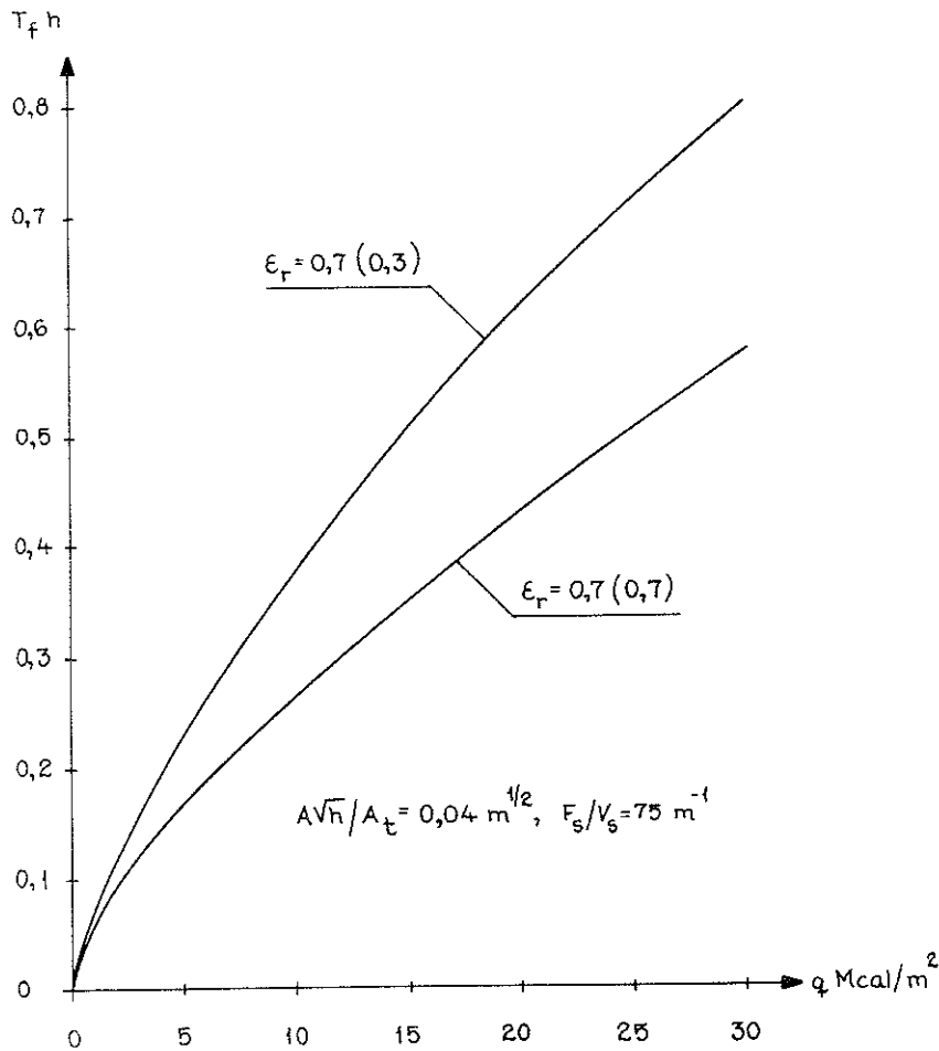
Fig. 18. Fictitious time of fire duration T_f at varying fire load q for a fire exposed, non-insulated steel structure. AV_h/A_t = 0.04 \text{ m}^{1/2} , F_s/V_s = 75 \text{ m}^{-1} . Both curves refer to a real fire exposure with a resultant emissivity \epsilon_r = 0.7 . As concerns the corresponding fire action according to the standard time-temperature curve, the upper curve presupposes a resultant emissivity \epsilon_r = 0.3 and the lower curve a resultant emissivity \epsilon_r = 0.7 .
