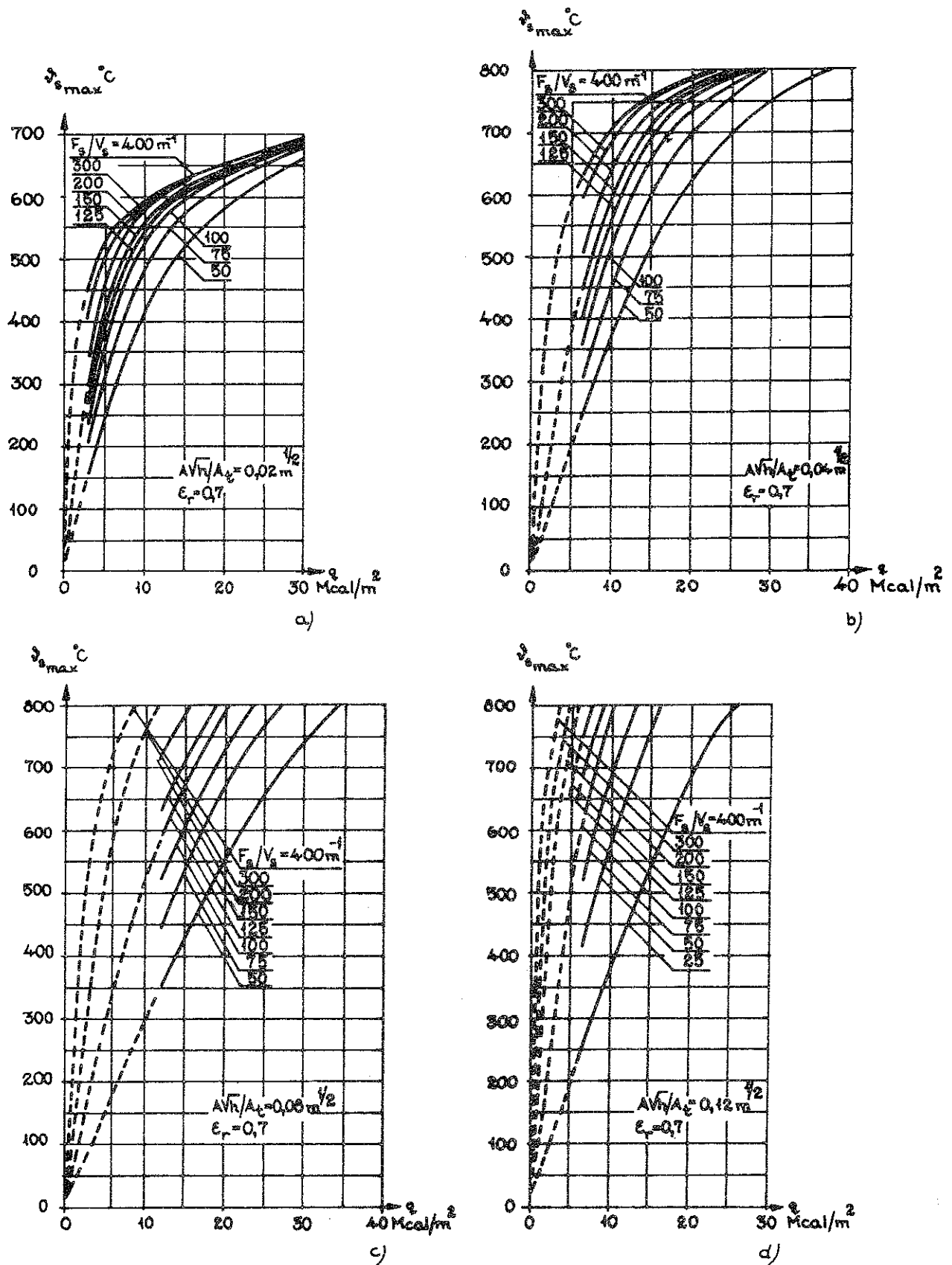
Fig. 8. Maximum steel temperature \vartheta_{s,max} for a fire exposed, non-insulated steel structure at varying opening factor AV_h/A_t , fire load q , and quotient F_s/V_s . \epsilon_r = 0.7 . The curves are based on fire characteristics according to Fig. 6 with the influence of the cooling phase taken into account [12], [13]
