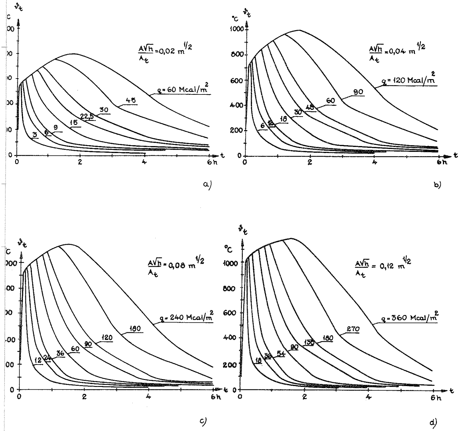
Fig. 6. Gastemperature-time curves ( \vartheta_t - t ) of the complete process of fire development for different values of the opening factor A\sqrt{h}/A_t ( \text{m}^{1/2} ) and the fire load q ( \text{Mcal/m}^2 of the total surface bounding the compartment). The curves correspond to a wood fire burning in a room enclosed by structures, 20 cm in thickness and made of a material with a thermal conductivity \lambda = 0.7 \text{ kcal/m}\cdot\text{h}\cdot^\circ\text{C} and a heat capacity \gamma_{c_p} = 400 \text{ kcal/m}^3\cdot^\circ\text{C} as representative average values within the temperature range actual [7]
