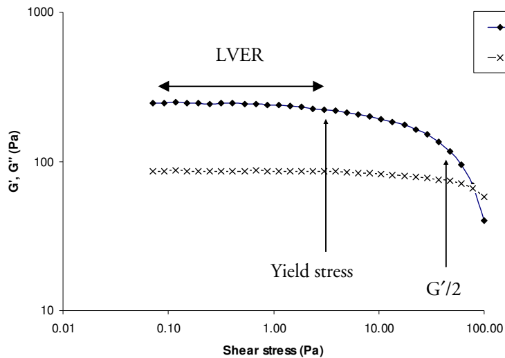
Figure 16. Rheogram of a 1.2% potato pulp suspension.
