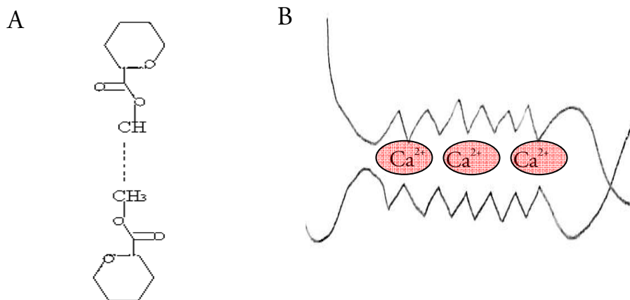
Figure 5. Gelling mechanism of pectin: A) hydrophobic interactions, B) Ca 2+ interactions
