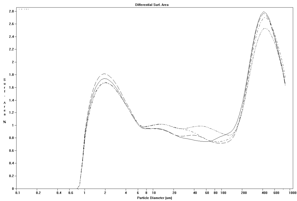
Figure 14. The surface-area-weighted particle size distributions of the differently heat-treated suspensions: HT0 (—), HT1 (---), HT2 (····) and HT3 (-·-·-) (see Table 3 for explanations). From Paper III.
