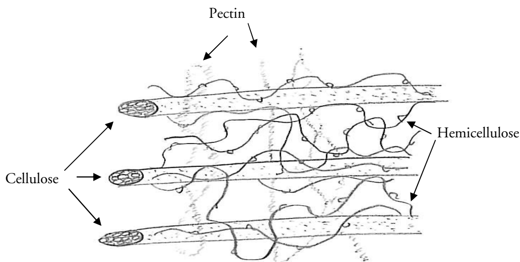
Figure 1. Schematic illustration of the cell wall (adapted from Carpita & Gibeaut [7]).
