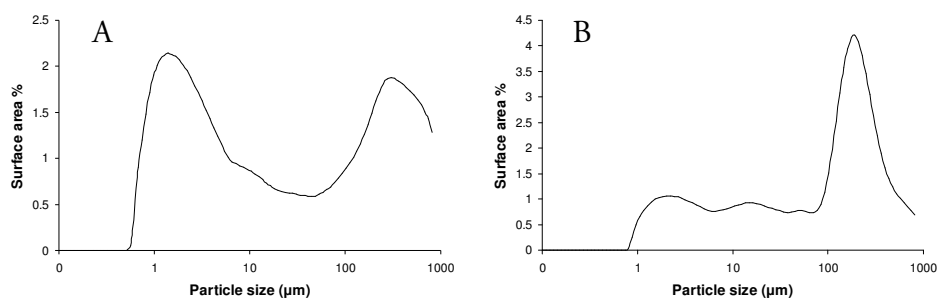
Figure 12. Surface-area-weighted particle size distributions of fibre suspensions. A) mainly bimodal distribution of potato pulp particles and B) mainly trimodal distribution of apple particles.
