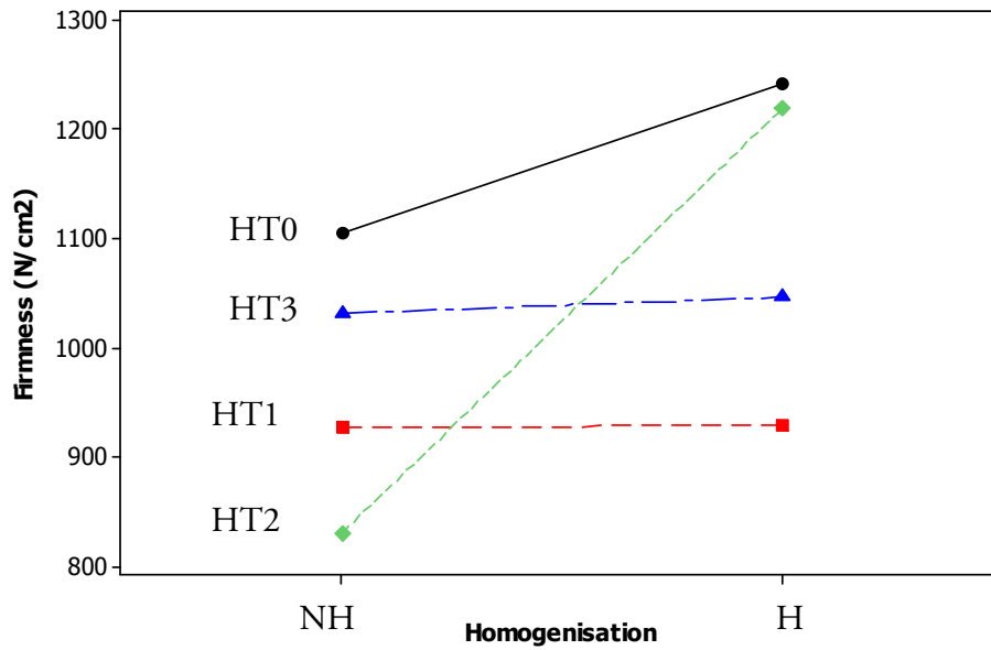
Figure 29. Interaction plots between homogenisation and heat treatment for firmness of sausages with potato pulp. NH = non-homogenised, and H = homogenised. Heat treatment: see Table 3. From Paper V.
