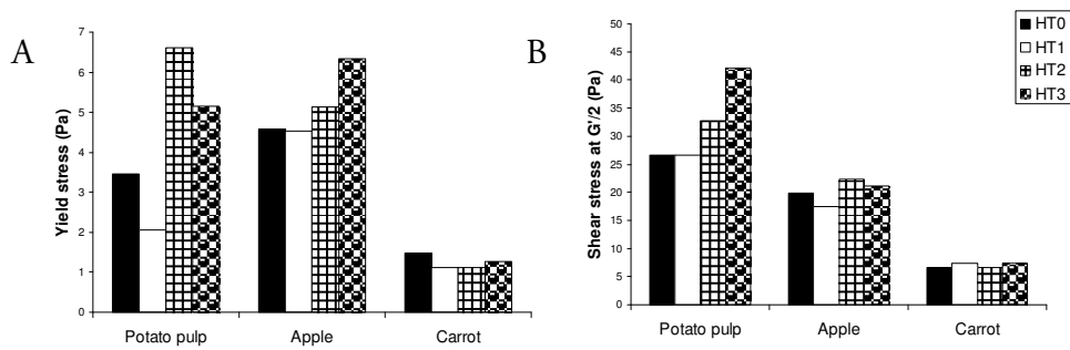
Figure 19. Yield stress (A) and shear stress at G'/2 (B) of three fibre suspensions at an IM concentration of 3% following heat treatment (see Table 3 for explanations)
