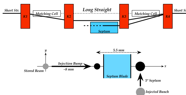
Figure 1: Conventional injection with a local bump in the MAX IV 3 GeV storage ring. Injection is displayed as seen from above (top) and in the transverse plane (bottom).
