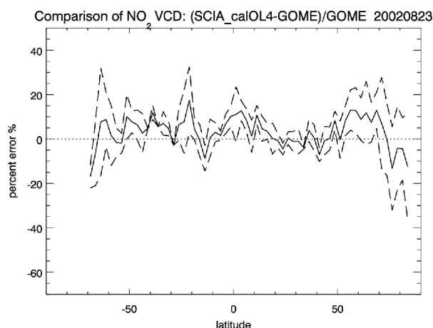
Figure 3 – Percent relative difference in total NO 2 between SCIAMACHY SCI_NL 5.01 and GOME GDP 3.0 along 2 orbits on August 23, 2002, plotted as a function of latitude.
