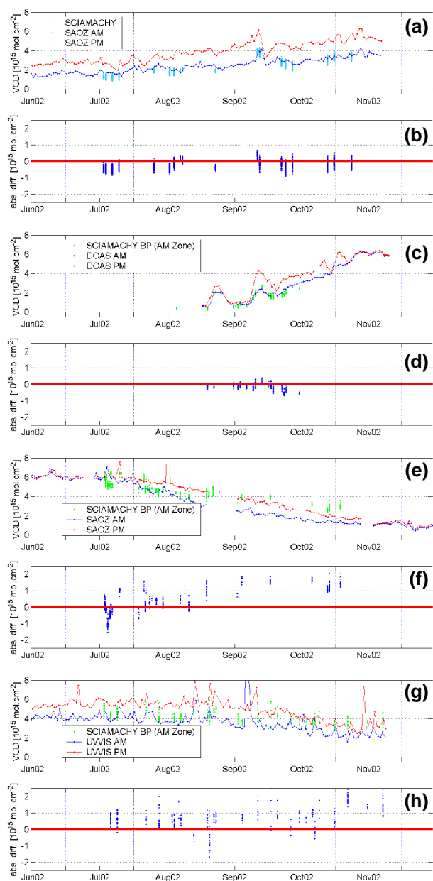
Figure 2 –Vertical column (a,c,e,g) of NO 2 from June to December 2002 as reported by SCIAMACHY v5.01 (mid-morning value) and by NDSC UV-visible spectrometers (sunrise and sunset values), and the absolute difference (b,d,f,h) SCIAMACHY – NDSC sunrise values at the following stations: (a-b) Kerguelen Island, 49°S, 70°E; (c-d) Neumayer, 71°S, 8°W; (e-f) Zhigansk, 67°N, 123°E; and (g-h) Monte Cimone, 44°N, 11°E.
