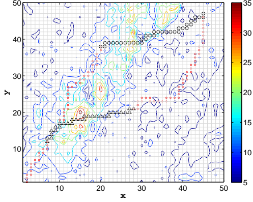
Figure 3.12: Contour plot of interpolated AGS eTh data (ppm) of the area from Paper IV. The cell size of the 50 \times 50 grid is 180 \times 180 m 2 . Two excerpts from the roads, referred to as route I (black triangles) and route II (black circles) are also plotted. Adapted from Paper IV.
