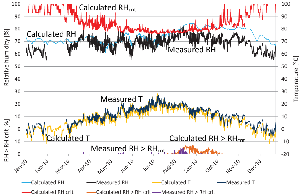
Figure 6: Folos 2D visual mould chart with comparisons of measured and calculated temperatures and RH in a construction [18]. Levels of RH crit from LIM I in Figure 1 [8]. Measured temperature (dark blue), calculated temperature (yellow), measured RH (black), calculated RH (turquoise), RH crit depending on calculated temperature (red), measured RH > measured RH crit (purple), calculated RH > RH crit (brown).
