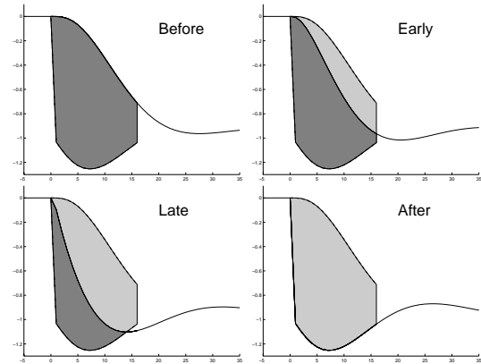
Fig. 3 The effect of a step disturbance for the different entry points in the process (as indicated in the figures). The indices were calculated to 1.0, 0.74, 0.36 and 0.0, in the order from before to after.
