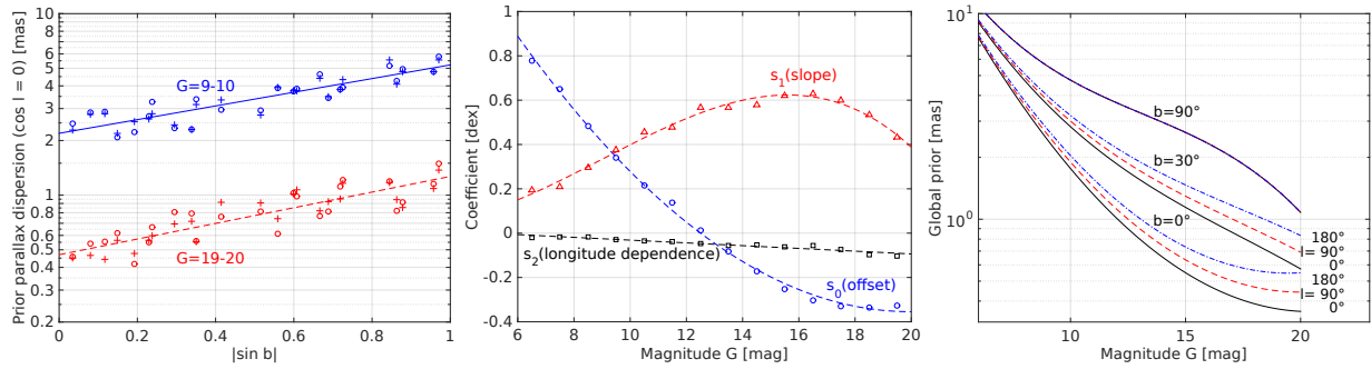
Fig. 4. Illustrations of the all-sky approximation to the parallax prior \sigma_{\pi,F90} as a function of galactic latitude b , for two magnitude ranges G = 9-10 (blue), and G = 19-20 (red). The small dependence on galactic longitude (the third term in Eq. (15)) has been subtracted leaving no systematic dependence on galactic longitude l , as shown by the different symbols ( \circ for \cos l > 0 , + for \cos l < 0 ). Middle: variations of the coefficients s_0 , s_1 , and s_2 with G magnitude, and polynomial fits according to Eqs. (16)–(18). Right: the prior \sigma_{\pi,F90} in Eq. (15) as a function of magnitude, for different latitudes (lowest to highest group: b = 0^\circ , 30^\circ , and 90^\circ ) and different longitudes (black solid l = 0^\circ , red dashed 90^\circ , blue dotted-dashed 180^\circ ).
