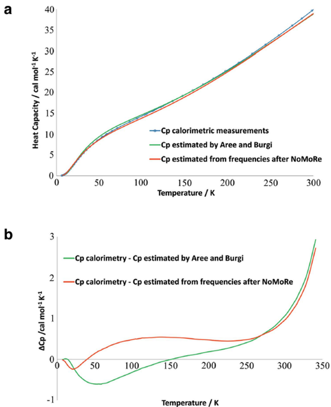
Figure 6. (a) Heat capacity ( C_p ) of naphthalene: from thermodynamic measurements (blue curve), calculated from frequencies obtained after NoMoRe (red curve) and estimated by Aree and B rgi (green curve), (b) difference between C_p from calorimetric measurements and C_p estimated by Aree and B rgi (green curve) and from NoMoRe (red curve). Reprinted from reference [173] under the general license agreement of IUCr journals.
