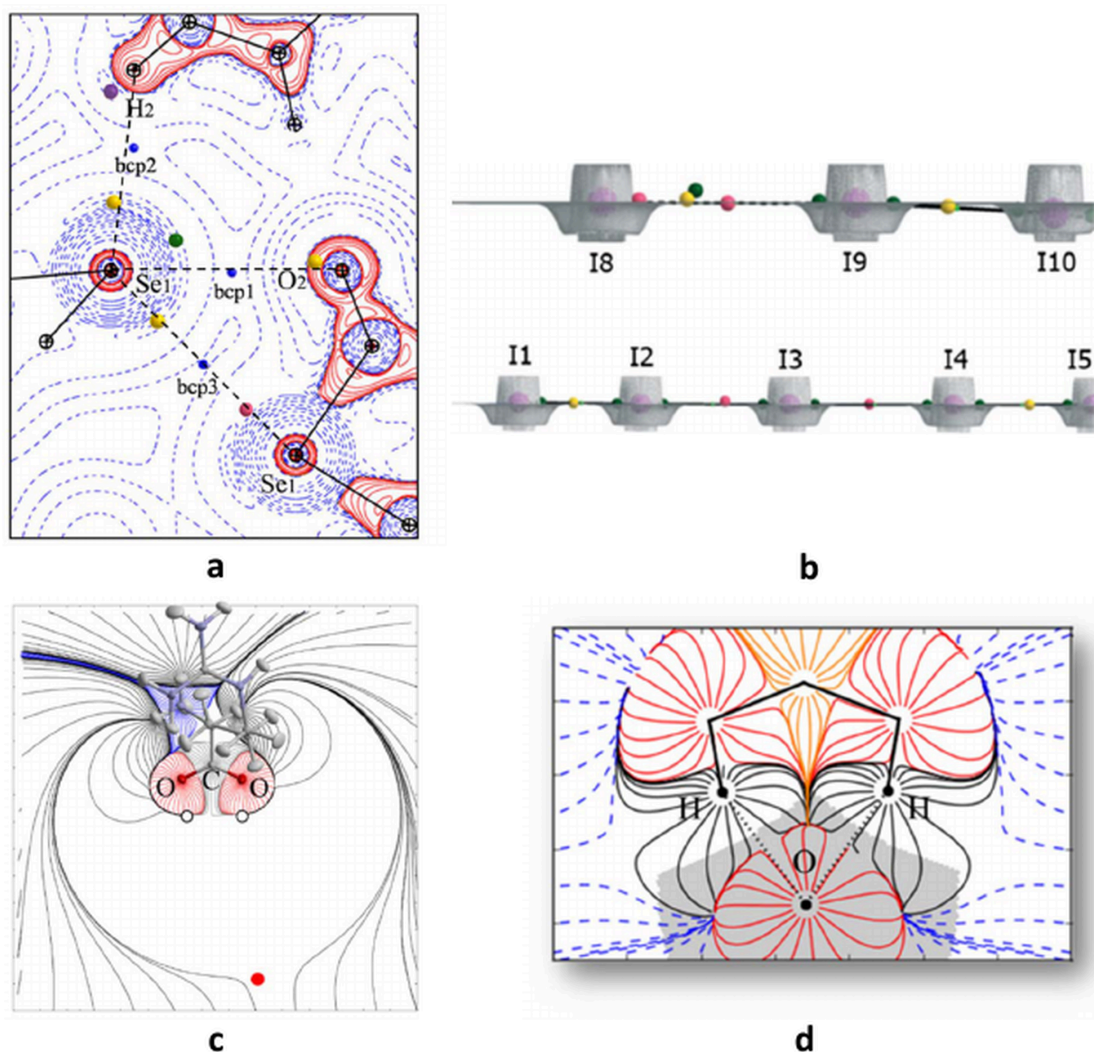
Figure 10. (a) L(\mathbf{r}) = -\nabla^2\rho(\mathbf{r}) experimental map in intermolecular regions of the \text{C}_8\text{O}_2\text{H}_4\text{Se} crystal structure: CC sites are represented by (3,-3) CPs of L (yellow spheres), CD sites are denoted by (3,+3) (violet), (3,+1) (pink) and (3,-1) (green) CPs of L . CC...CD directions closely correspond to internuclear directions (dashed lines), which in turn almost superimpose with bond path directions (bond critical points are in blue). (b) CPs of L(\mathbf{r}) = -\nabla^2\rho(\mathbf{r}) in two regions of a poly-iodide chain (same color-code used in (a)): covalent bonds are identified by (3,-3) CPs in the middle of the bonds of I1-I2, I4-I5 and I9-I10, while intermolecular interactions are characterized by (3,+1) CPs in the middle of I2...I3...I4 and I8...I9 regions. I9 is an iodine atom making a type-II halogen bonding interaction with iodine I8 (I8(CC)...(CD)I9) and a covalent interaction with I10, whereas I3 is an iodide displaying non-covalent interactions with both I2 and I4 iodine. (c) Experimental gradient vector field of V(\mathbf{r}) for the L-histidinium cation in the crystal structure of L-histidinium phosphate phosphoric acid: the influence zone of its nucleophilic COO-group is limited by a zero-flux surface of V(\mathbf{r}) , the distance up to the saddle point in the surface ((3,+1) CP, red sphere) being approximately 6 Å. (d) At the equilibrium geometry of the phosphate...phosphate complex, the O-atomic basin (grey region) lays within the influence zones (electrostatic basins) of the H-nuclei. Black \epsilon(\mathbf{r}) lines crossing the region between the zero flux surfaces of \rho(\mathbf{r}) (grey border) and V(\mathbf{r})
