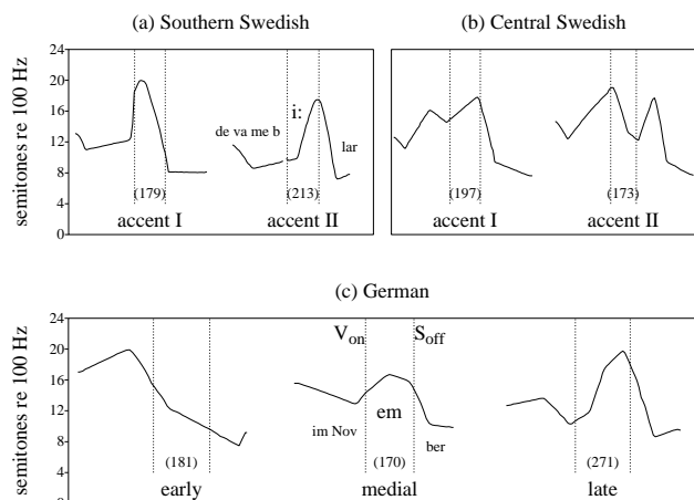
Figure 1: Typical realisations of the Swedish word accents I and II in (a) Southern and (b) Central Swedish, compared to (c) the three-fold contrast of sentence-level pitch accents in German. Stylised F_0 -curves based on authentic productions of a short phrase: Swedish accent I (a&b): det var med bilen ‘by car’; Swedish accent II (a&b): det var med bilar ‘with cars’; German (c): im November ‘in November’. Dotted lines delimit the rhyme of the stressed syllable (in parentheses: duration in ms); V_{on} = stressed vowel onset; S_{off} = stressed syllable offset.
