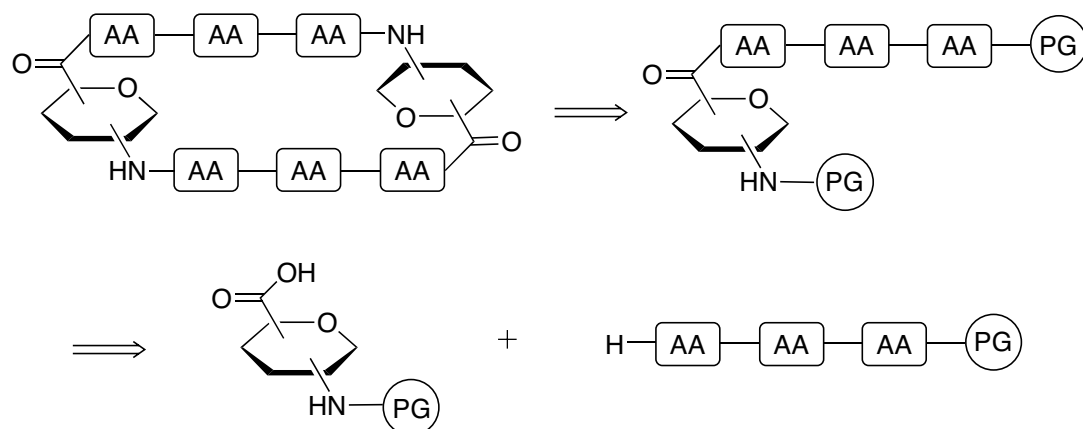
Figure 5.1 General structure and retrosynthetic analysis of the synthetic targets.
