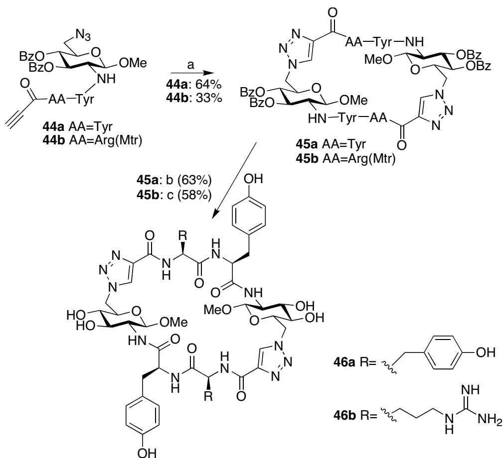
Scheme 7.5 Cyclization and deprotection. Reaction conditions: (a) CuI/DIPEA/THF, 45 °C; (b) NaOMe/MeOH, 24 h; (c) TFA/PhSMe, 24 h; (d) NaOMe/MeOH, 48 h.
