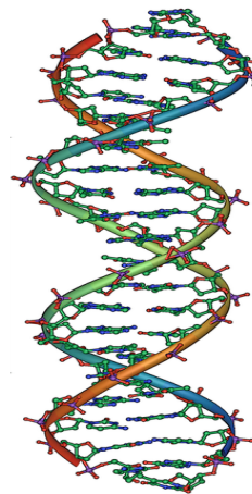
Figure 2.3: The double-helix DNA giant molecule. Picture taken from ref. [8]
