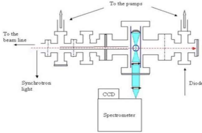
Figure 3.3: Experimental setup. The synchrotron light comes into the chamber from the left and continues to the right through a small capillary, the interaction zone and to the diode. The fluorescence coming from the interaction zone is gathered by an optical system and focused to the slit entrance of the spectrometer. Two ports of the chamber are connected to two pumps which maintain the vacuum inside [9].
