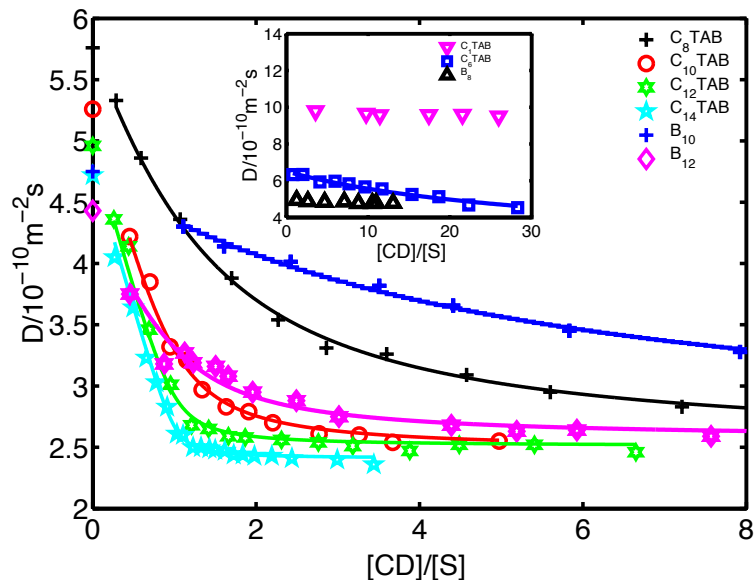
Figure 5.4 Self-diffusion coefficients for n-akyltrimethylammonium bromide surfactants and bolaform surfactants plotted versus the ratio of [\beta\text{-CD}]/[\text{S}] at 298 K. The concentration of the surfactants are: [\text{C}_1\text{TAB}] = 0.43 \text{ mM} , [\text{C}_6\text{TAB}] = 0.47 \text{ mM} , [\text{C}_8\text{TAB}] = 1.6 \text{ mM} , [\text{C}_{10}\text{TAB}] = 2.0 \text{ mM} , [\text{C}_{12}\text{TAB}] = 2.0 \text{ mM} , [\text{C}_{14}\text{TAB}] = 3.5 \text{ mM} , [\text{B}_8] = 1.1 \text{ mM} , [\text{B}_{10}] = 0.98 \text{ mM} and [\text{B}_{12}] = 1.0 \text{ mM} .
