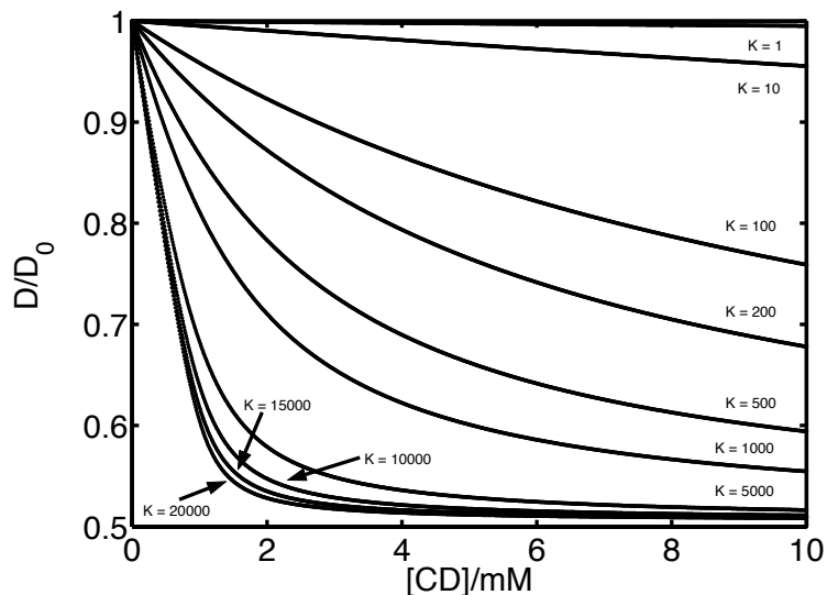
Figure 4.6 Simulated normalized self-diffusion data versus [CD] for a 1:1 complexation. It can be seen that with increasing K_{11} the curves initial slope become insensitive towards high values of K_{11} . The curves in the graph are calculated based on a concentration of guest molecules of 1 mM and the D_{S,f} = 4.96 \cdot 10^{-10} \text{ m}^2 \text{ s}^{-1} , D_{CD,f} = 2.64 \cdot 10^{-10} \text{ m}^2 \text{ s}^{-1} and D_{CD-S} = 2.51 \cdot 10^{-10} \text{ m}^2 \text{ s}^{-1} (i.e. realistic values).
