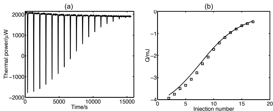
Figure 5.7 (a) Thermal power as a function of time for sequential 4.16 \mu L injections of 0.1116 mol \text{kg}^{-1} B_{12} into 4.746 mmol \text{kg}^{-1} \beta -CD aqueous solution at 308.20 K. (b) Heat ( Q ) per injection versus injection number at 308.20 K, ( \square ) are experimental points and (—) fitted line.
