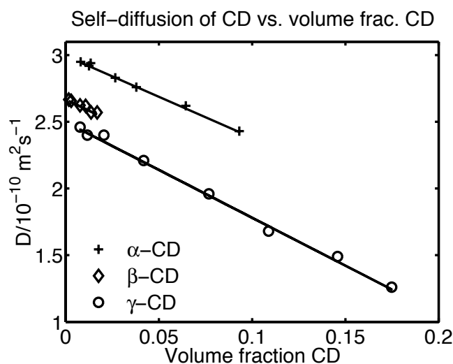
Figure 2.5 Self-diffusion coefficients versus volume fraction of cyclodextrin.
