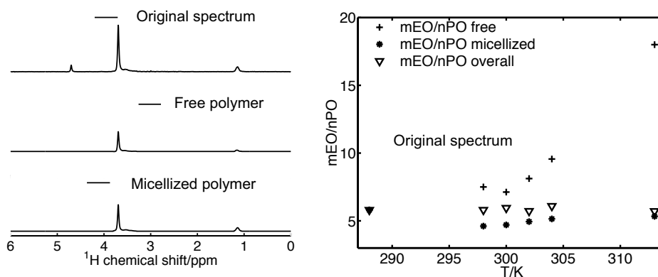
Figure 7.2 (a) CORE approach applied to separate overlapping peaks for F127 at 1 wt% at 302K. (b) Ratio between the numbers of EO units (m) to PO units (n) versus T . The case of free micellized, and overall are shown.
