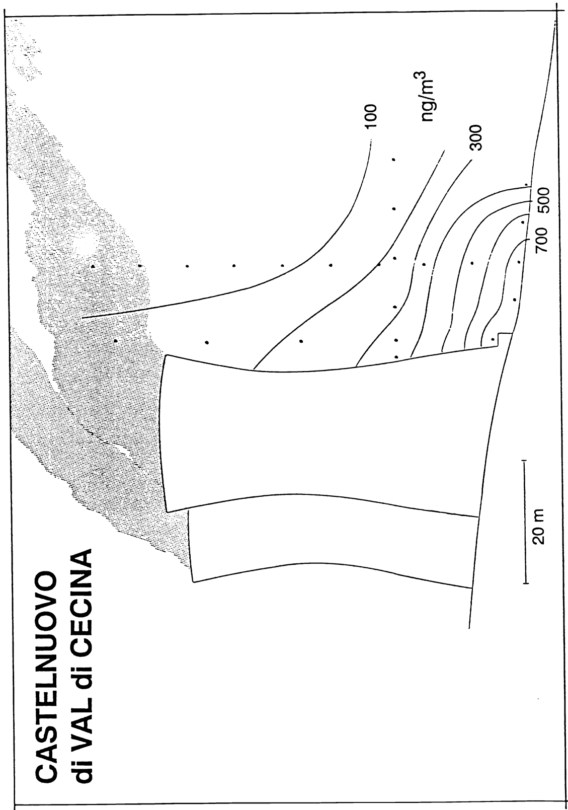
Figure 3. Hg mapping close to the cooling towers at a geothermal power plant, Hg concentrations in \text{ng}/\text{m}^3 .
