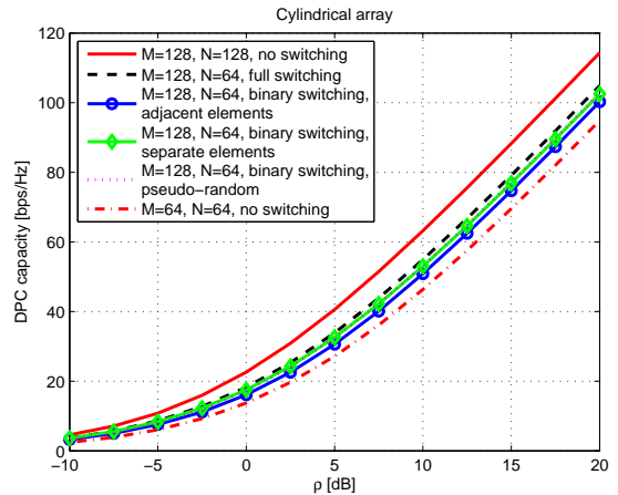
Fig. 10. Performance comparison in the scenario where sixteen users are distributed at MS 1-8, half have LOS conditions and half have NLOS conditions, with the cylindrical array at the base station.
