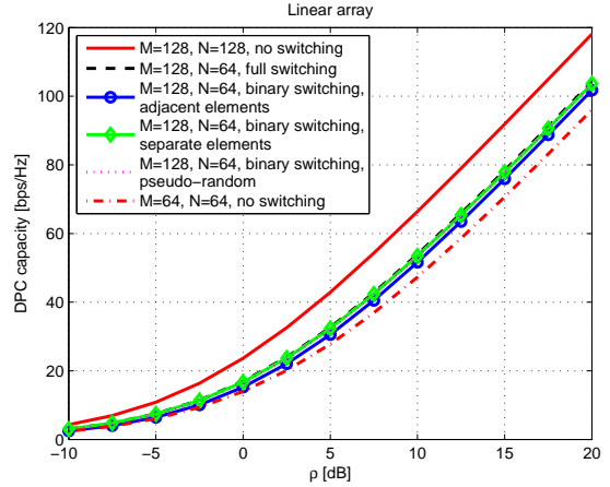
Fig. 9. Performance comparison in the scenario where sixteen users are distributed at MS 1-8, half have LOS conditions and half have NLOS conditions, with the linear array at the base station.
