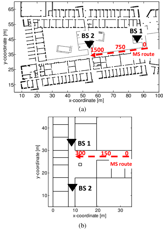
Fig. 2. Floor plan of the measurement environment with transmitter routes and receiver positions. (a) Indoor hall scenario in Computer Science building. (b) Office corridor scenario in Department of Radio Science and Engineering. Both buildings are located in Aalto University School of Science and Technology, Helsinki, Finland.
