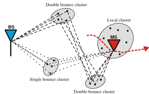
Fig. 1. Example of a GSCM. The black dots inside each cluster depict the individual MPCs.
