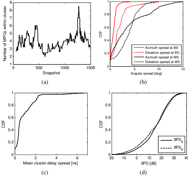
Fig. 4. (a) Number of MPCs within clusters. (b) Cluster angular spread. (c) Cluster delay spread. (d) Cross-polarization discrimination. All parameters have been extracted from the reference measurement.
