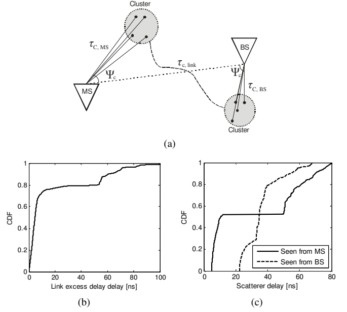
Fig. 5. (a) Parameters defining the locations of the clusters. CDFs of the (b) link excess delay and (c) scatterer delay. All parameters have been extracted from the reference measurement.
