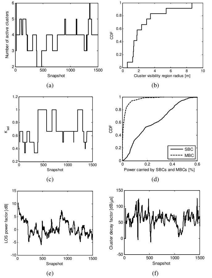
Fig. 3. (a) Total number of active clusters as a function of the MS location. (b) CDF of the visibility region radius. (c) Ratio of single and multiple bounce clusters. (d) Power carried by SBCs and MBCs. (e) LOS power factor. (f) Cluster decay factor. All parameters have been extracted from the reference measurement.
