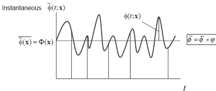
Figure 15. The curved line in the diagram illustrates how the position of a flame fluctuates over time. \bar{\phi} represents the mean value of the flame position over time, \varphi is the change in fluctuation and \tilde{\phi} is the instantaneous position of the flame.
