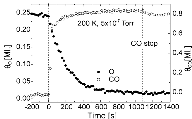
FIG. 7. Time evolution of \theta_{\text{O}} and \theta_{\text{CO}} at a relatively high CO pressure ( T=200 K, P_{\text{CO}}=5 \times 10^{-7} Torr). The absence of the induction period is due to quick CO adsorption under this condition. CO exposure was ceased at 1080 s.
