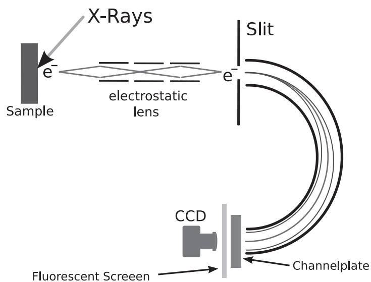
Figure 6.6: Schematic representation of a hemispherical electron analyser using a CCD based multichannel detector.
