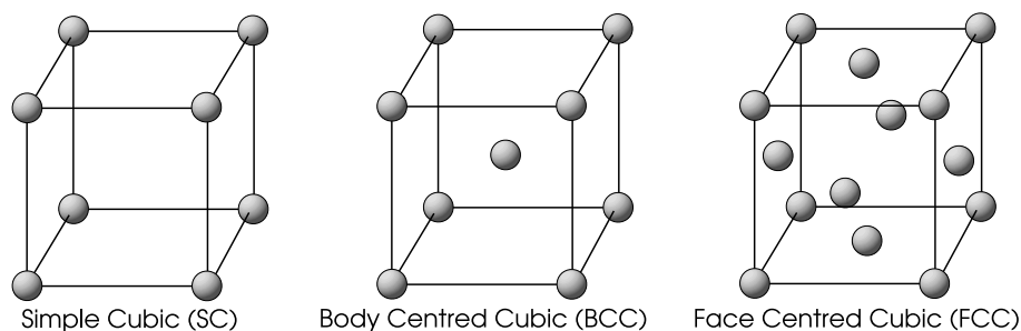
Figure 2.1: Cubic structures.
