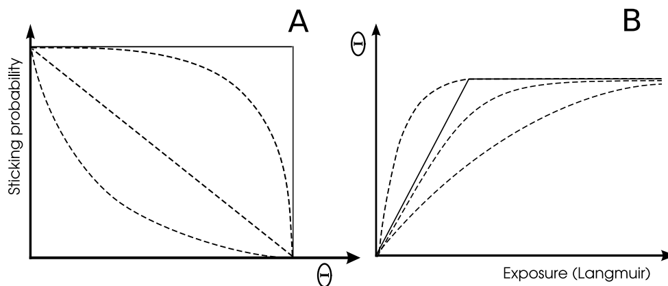
Figure 4.3: A) Shows the sticking probability versus the coverage. The described adsorption behaviours are only qualitative: solid line: constant up to \Theta_{\max} , zero thereafter. Dashed line: \propto (1 - \Theta) . Dash-dotted line: limited mobility precursor. Dotted line: dissociative adsorption. In B) is shown the resulting coverage versus Langmuir exposure.
