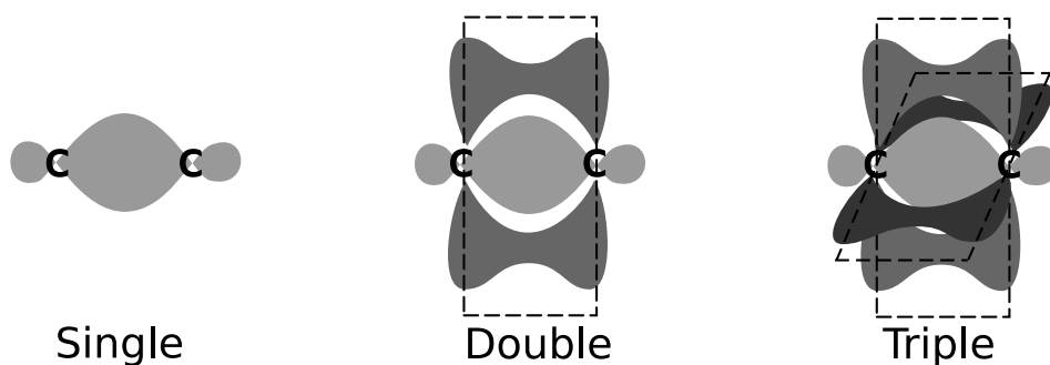
Figure 3.3: Schematic picture illustrating the three bond orders between two carbon atoms. From the left: single bound as in H_3CCH_3 (Ethane), double bond as in H_2CCH_2 (Ethene), triple bond as in HCCH (Ethyne).
