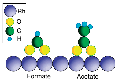
Fig. 4. Schematic adsorption geometry for formate and acetate on the Rh(111) surface.
