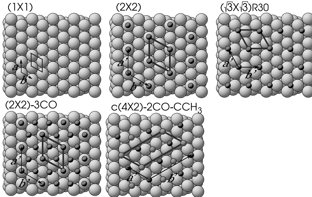
Figure 2.4: Some examples of how adsorbate structures are described in terms of the FCC (111) (1×1) unit cell. The (2×2)-1CO has been found for both oxygen and CO adsorbed on Rh(111). The (2×2)-3CO represents the Rh(111) CO surface saturation. The (\sqrt{3}\times\sqrt{3})R30^\circ -1O is one of the reactive oxygen compressed phases found on Pd(111). The c(4\times 2) -2CO-2C 2 CH 3 has been found for ethynidyne co-adsorbed with CO on Rh(111). All these phases are relevant to this thesis.
