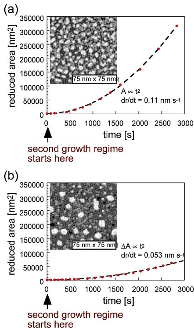
Figure 7. Growth of a single reduced patch at 1 \times 10^{-7} \text{ mbar H}_2 for (a) the normal preparation of the oxide and (b) a smoother surface oxide created by removal of 0.21 ML before oxidation. Surface b has fewer domain boundaries, fewer islands, but slightly more holes (inset).
