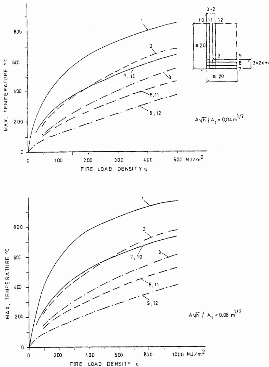
FIG 6. Maximum temperature in different points of a concrete beam of rectangular cross section, fire exposed from below on three sides. Fire exposure according to FIG 5, differentiated with respect to the fire load density q and the opening factor A\sqrt{h}/A_t of the fire compartment.
