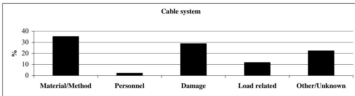
Figure 2, Failure statistics of cable systems 2005 [18]
