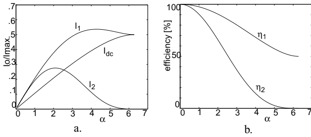
Fig. 2. a). Ideal normalized DC, fundamental and second order output current as function of the conduction angle \alpha , b). drain efficiency for the fundamental and second-order output.
