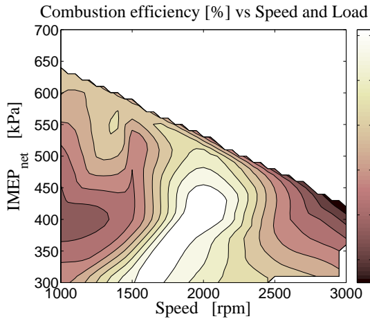
Figure 32: Combustion efficiency
