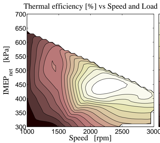
Figure 33: Thermal efficiency
