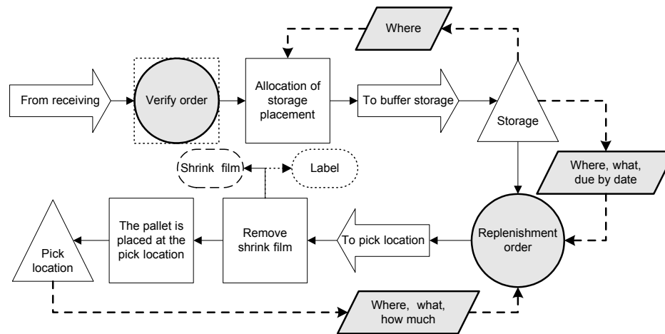
Figure 5.5. The storing process at distribution centres incorporating RFID technology
