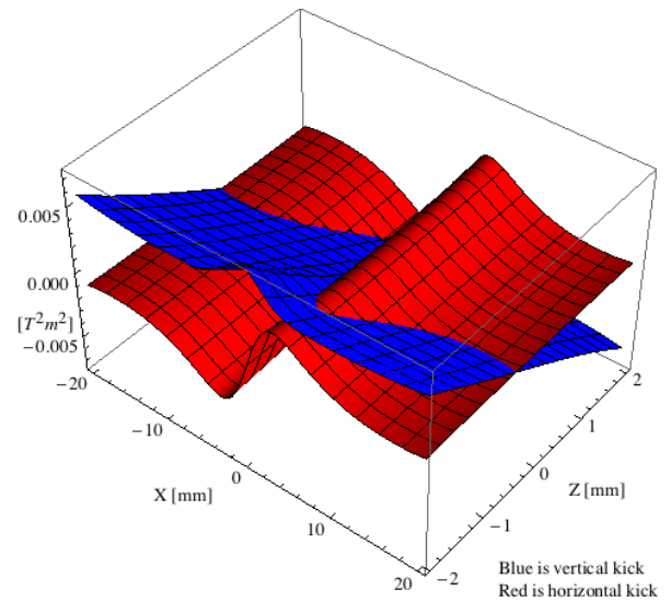
Figure 1: Kick map of epu53 in helical mode.
