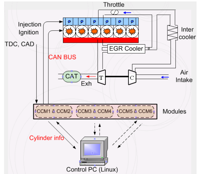
Figure 1: The Engine and its control system
